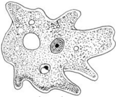
Amoeba
